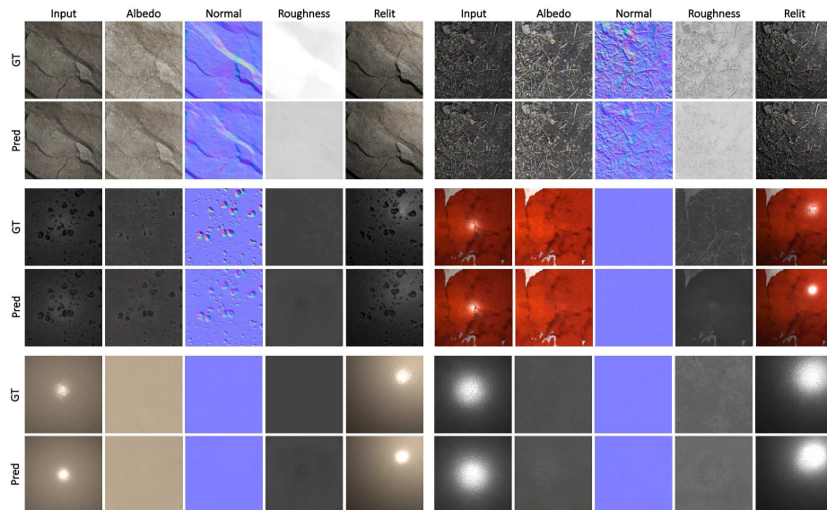
Fig. 4. BRDF reconstruction results from our full method ( c1sCRF-pt in Table 3) on the test set. We compare the ground truth parameters with our reconstructions as well as renderings of these parameters under novel lighting. The accuracy of our renderings indicates the accuracy of our method.
