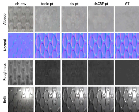
Fig. 6. Qualitative comparison of BRDF reconstruction results of different variants of our network. The notation is the same as Table 3 and -env represents environment illumination.
