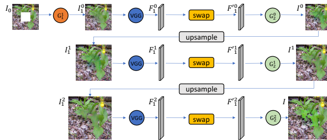
Fig. 4. Multi-scale inference.
