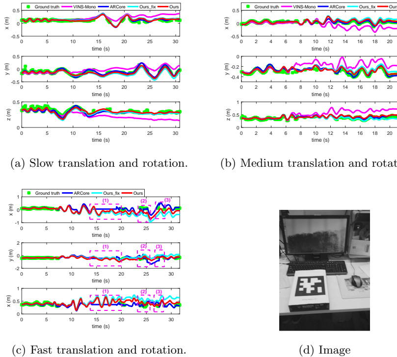
Fig. 8: The qualitative comparison of tracking accuracy. VINS-Mono fails to track on the fast translation and rotation sequence.
