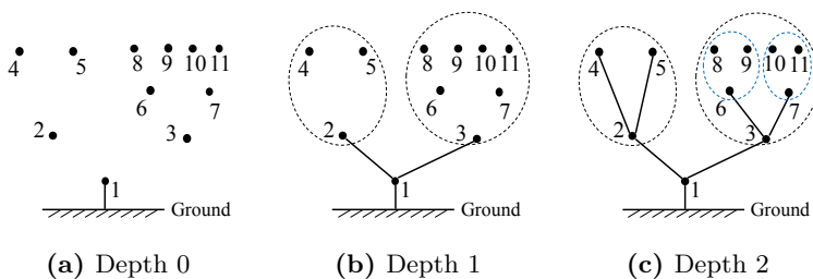
Fig. 5. Illustration of our hierarchical clustering algorithm. See Section 4.2 for details. term for the distance on the graph from i to the origin, and the secondary key d_i is the Chebyshev ( L_\infty ) distance between i to the center of its closure.
