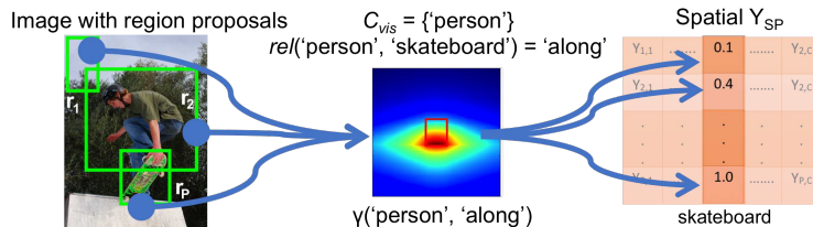
Fig. 7. Spatial Common-sense: The Y_{sp}(., skateboard) values are computed by measuring the spatial relationship of proposals with respect to the source ‘person’ class. Based on our knowledge base [19], ‘along’ is the most common relation between the ‘skateboard’ and ‘person’ class. Observe that the proposal r_p gets the highest Y_{sp} value.
