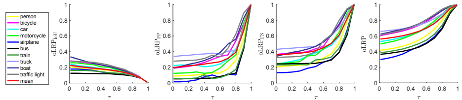
Fig. 3: For each class, oLRP and its components for Faster R-CNN (X101+FPN) are plotted against \tau . The mean represents the mean of 80 classes.
