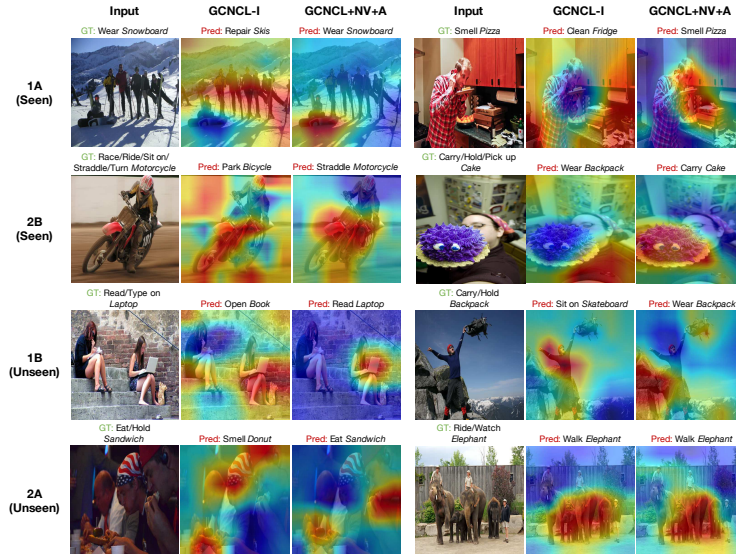
Fig. 3. Results of GCNCL-I and GCNCL+NV+A on HICO dataset. All methods are trained on 1A+2B and tested on both seen (1A, 2B) and unseen (2A, 1B) actions. Each row shows results on a subset. Each sample includes the input image and its label, top-1 predictions from GCNCL-I and GCNCL+NV+A. We plot the attention map using the top-1 predicted labels. Red regions correspond to high prediction scores.
