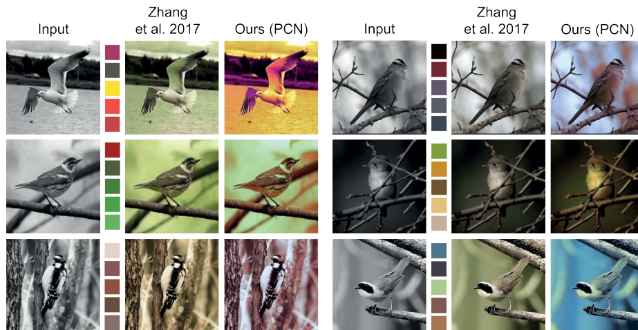
Fig. 10. We compare colorization results with previous work [44]. The five-color palette used for colorization is shown next to the input grayscale image. Note that our PCN performs better at applying various colors included in the palette.
