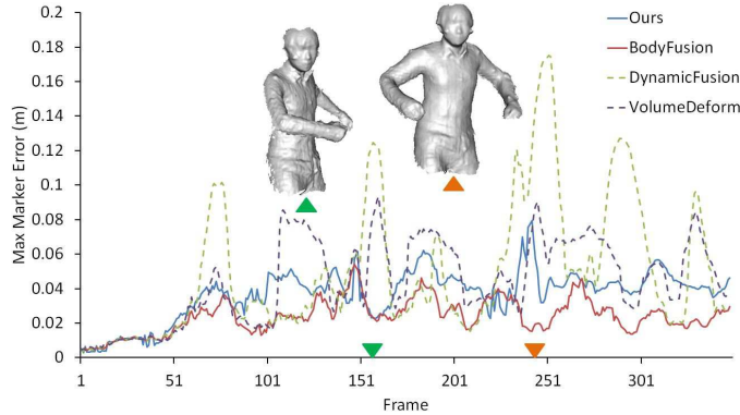
Fig. 9. Quantitative comparison: max marker errors of our method, BodyFusion, DynamicFusion and VolumeDeform for a motion sequence.
